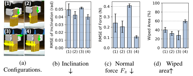
Fig. 7: Comparison of different sensor configurations. : (1) proximity sensors inside the finger, (2) a single proximity sensor, (3) normal force only, (4) proposed shear and slip force with an array of proximity sensors.
