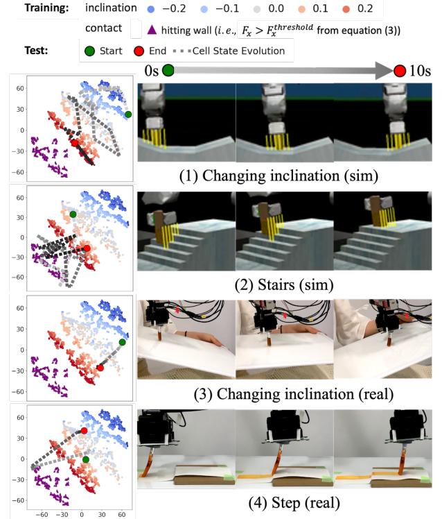
Fig. 8: The t-SNE visualisation of cell state evolution in the feature extraction module over time and the adaptation of robot motion on the fly in simulated and physical setups.
