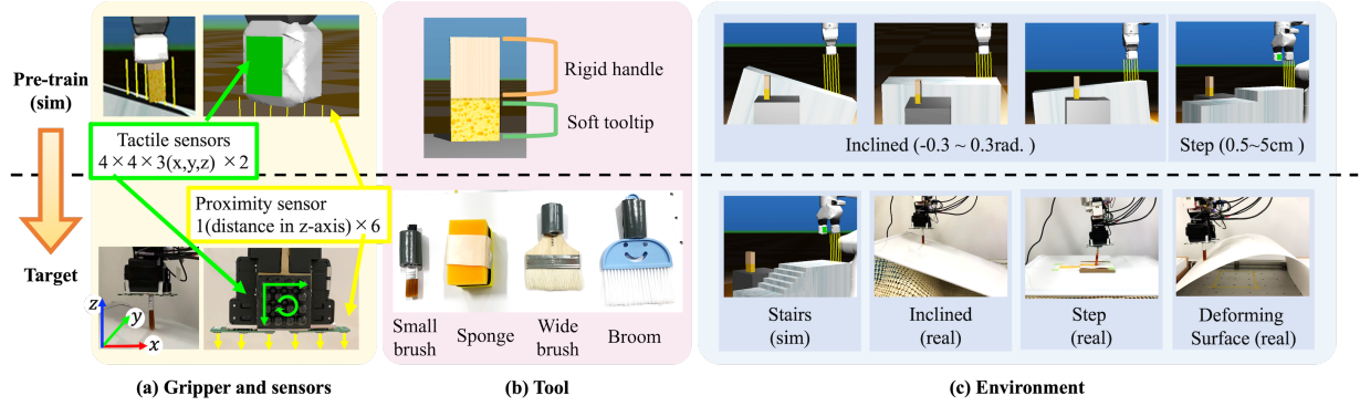
Fig. 4: Experimental setup.
