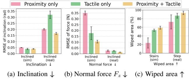
Fig. 6: Contribution of each modality.
